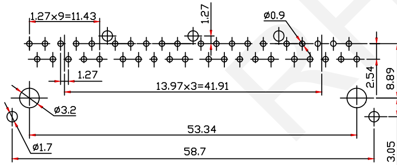
PCB Layout
